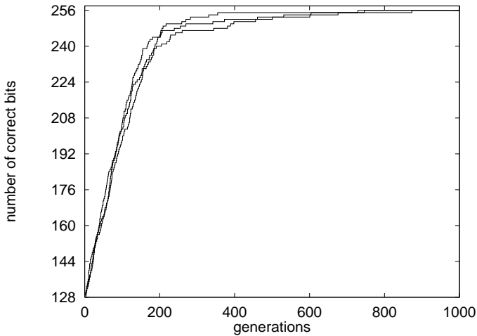
Fig. 7. Number of correct bits corresponding to Fig. 6.
