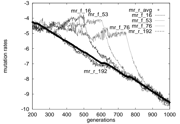
Fig. 8. Self-adaptation of three mutation rates responsible for bits with a starting value of ‘0’ ( mr - f_* ), of the average mutation rate of those bits initialized correctly ( mr - r_{avg} ) and one mutation rate responsible for a bit with a correct starting value ( mr - r_{192} ).
