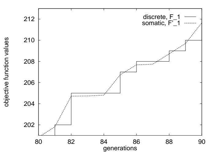
Fig. 4. Zoom into a single run of a (15, 100) ES solving the COP.
