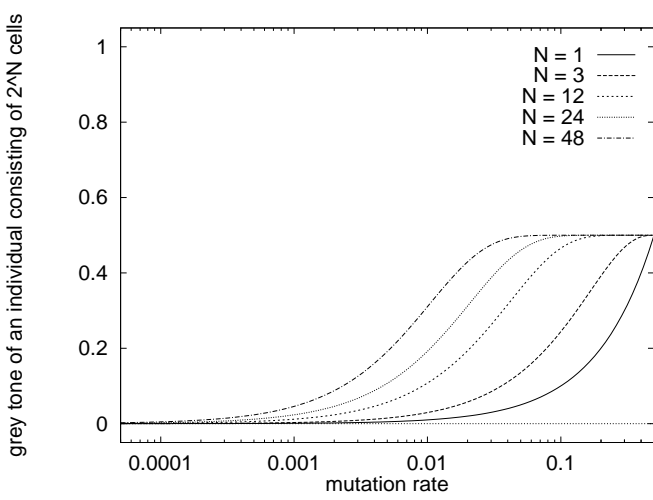
Fig. 2. Intermediary grey tone values derived from the mutation rates (bonus only) for different numbers N of cell divisions.
