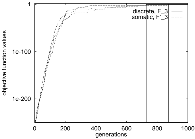
Fig. 6. 3 runs of a (15,100) ES solving F_3 .
