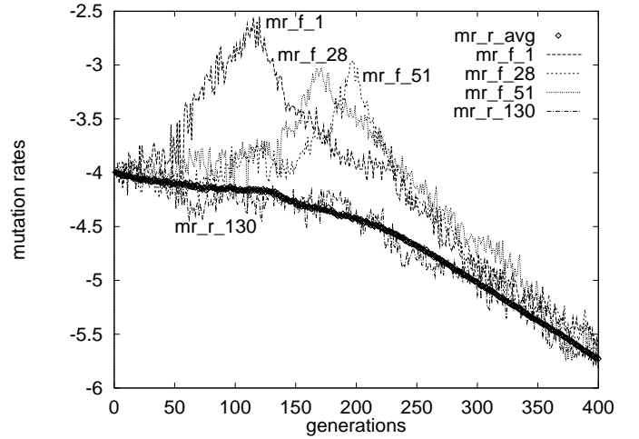
Fig. 5. Self-adaptation of three mutation rates responsible for bits with a starting value of '0' ( mr_f^* ), of the average mutation rate of those bits initialized correctly ( mr_r_{avg} ) and one mutation rate responsible for a bit with a correct starting value ( mr_r_{130} ).
