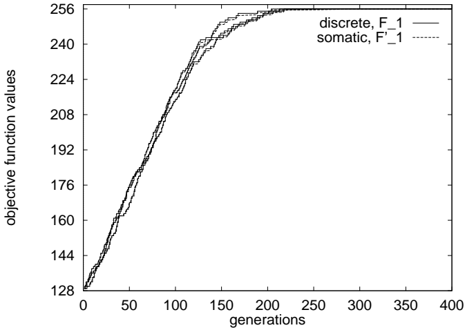
Fig. 3. 3 runs of a (15, 100) ES solving the COP.
